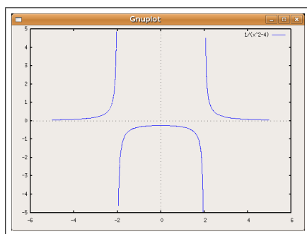
(a) \frac{1}{x^2-4} , "set zero axis;"
