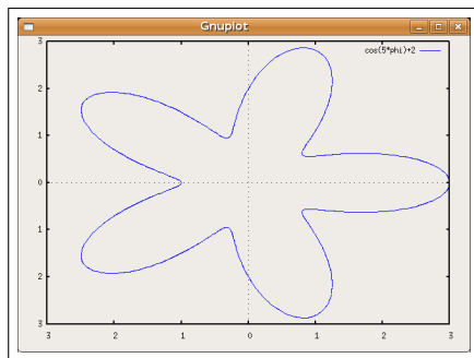
(c) r(\phi) = 2 + \cos(5\phi) , "set polar"
