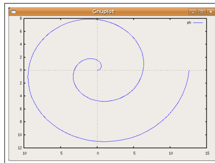
(b) r(\phi) = \phi , "nticks, 30"
