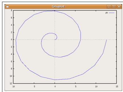
(a) r(\phi) = \phi
