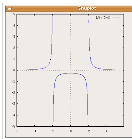
(b) \frac{1}{x^2-4} , "set size ratio 1; set zero axis;"
